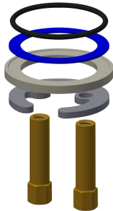
Quick-action fastener
